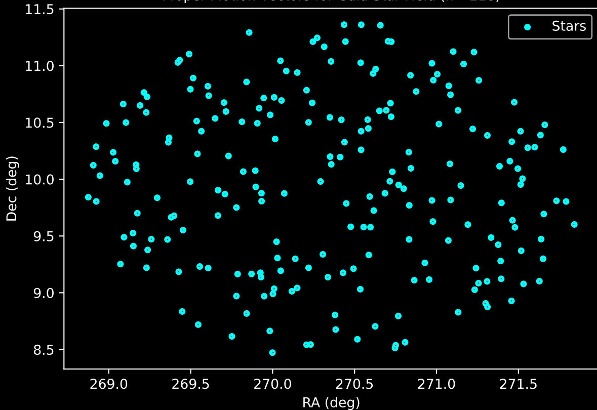
APOGEE DR17 Field: [247+62_btx] Proper Motion Vectors for Gaia Star Field (n= 218)
