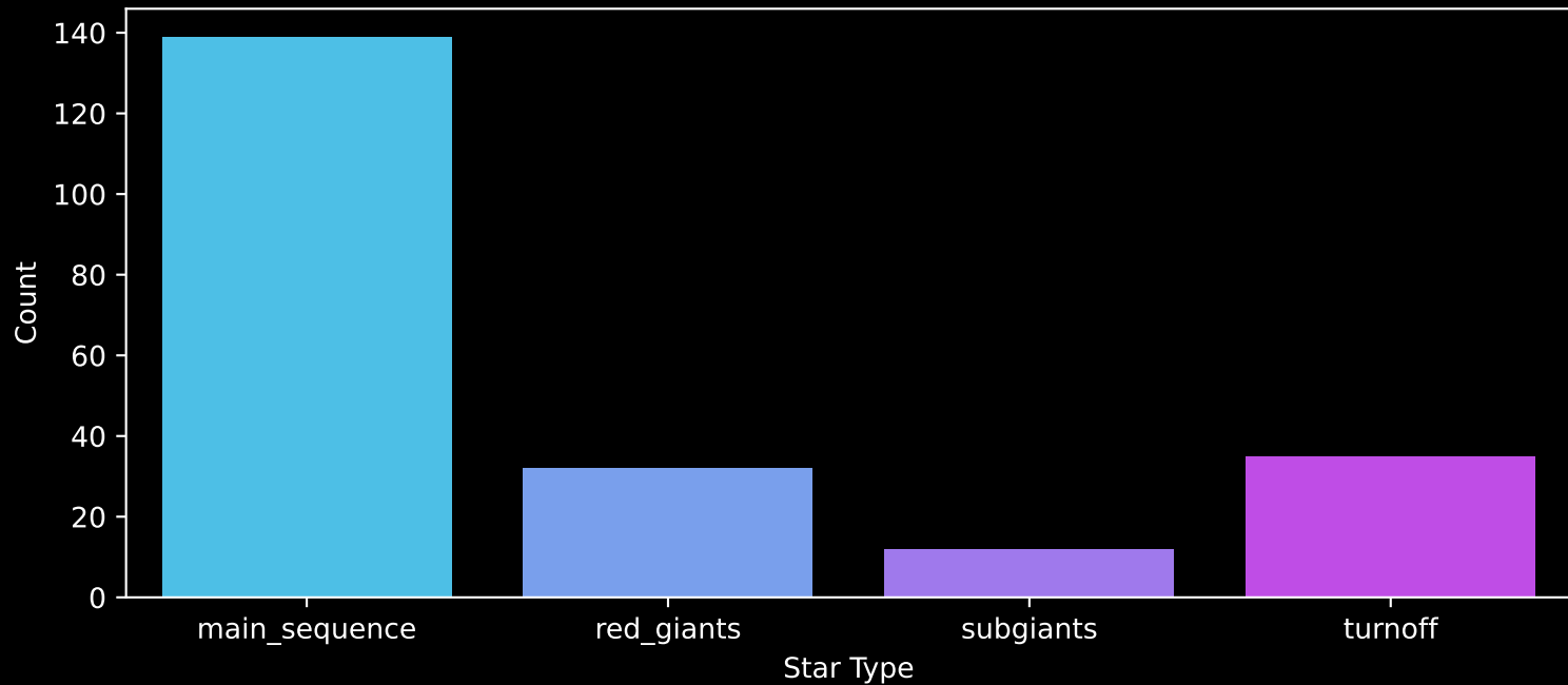
APOGEE DR17 Field: [247+62_btx] Count plot of Star Type
