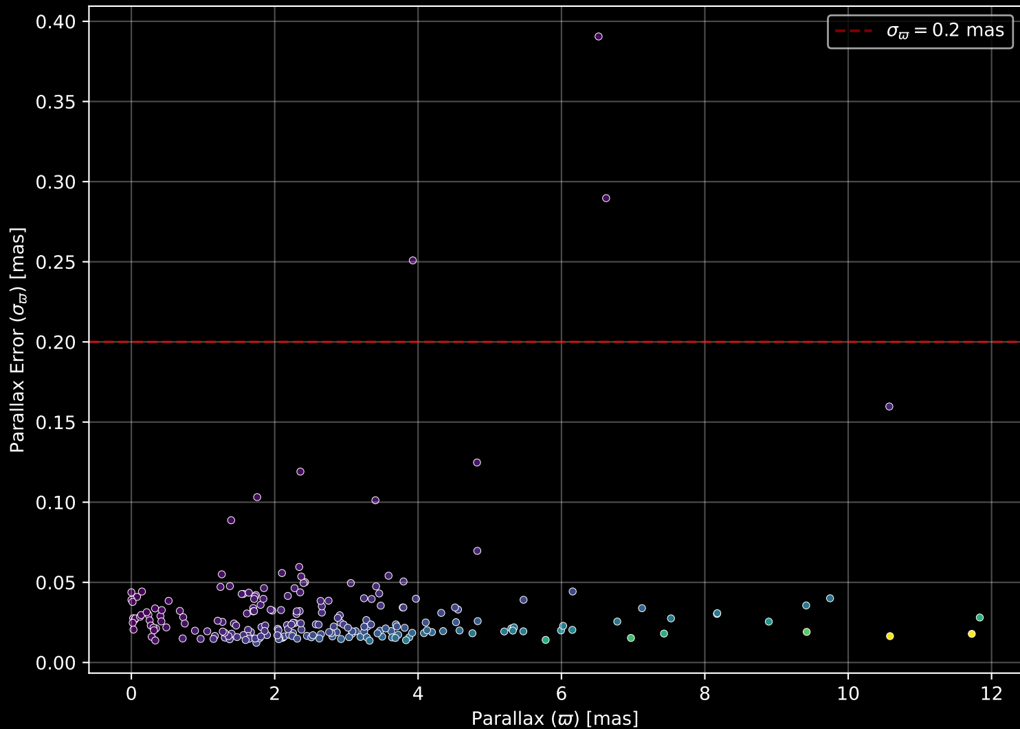
APOGEE DR17 Field: [247+62_btx] Parallax Quality (n= 218)
