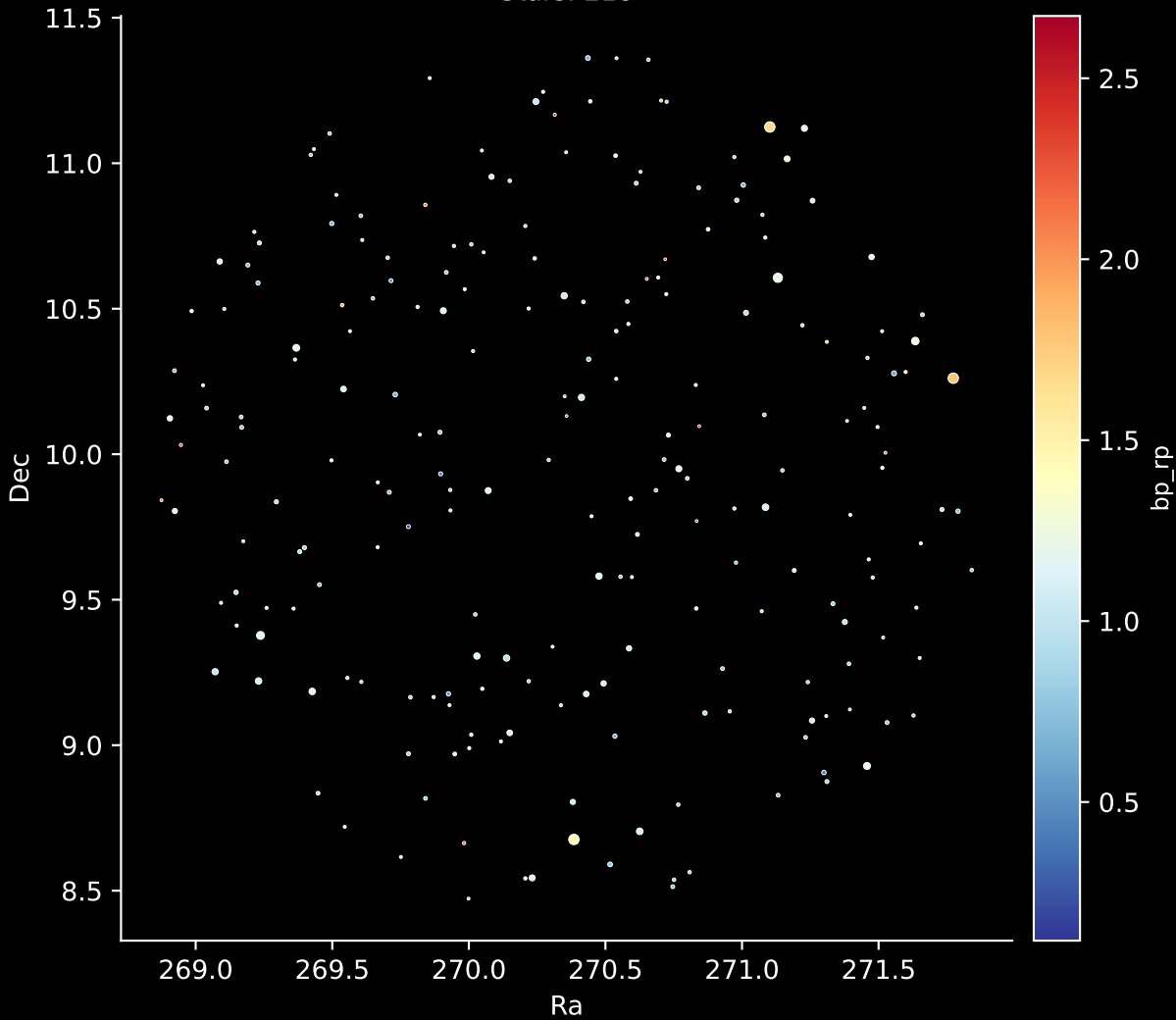
APOGEE DR17 Field: [247+62_btx] Stars: 218
