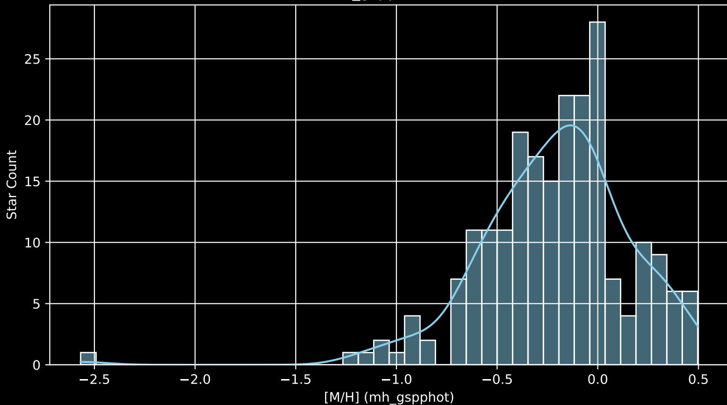
APOGEE DR17 Field: [247+62_btx [M/H] (mh_gspphot) (n= 217)
