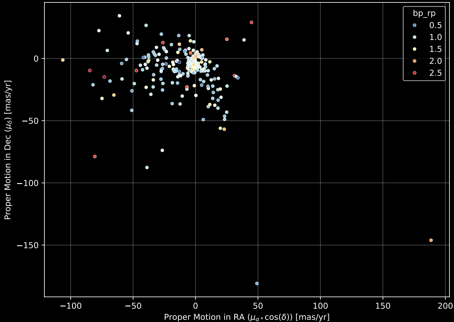
APOGEE DR17 Field: [247+62_btx] Proper Motion Diagram (n= 218)
