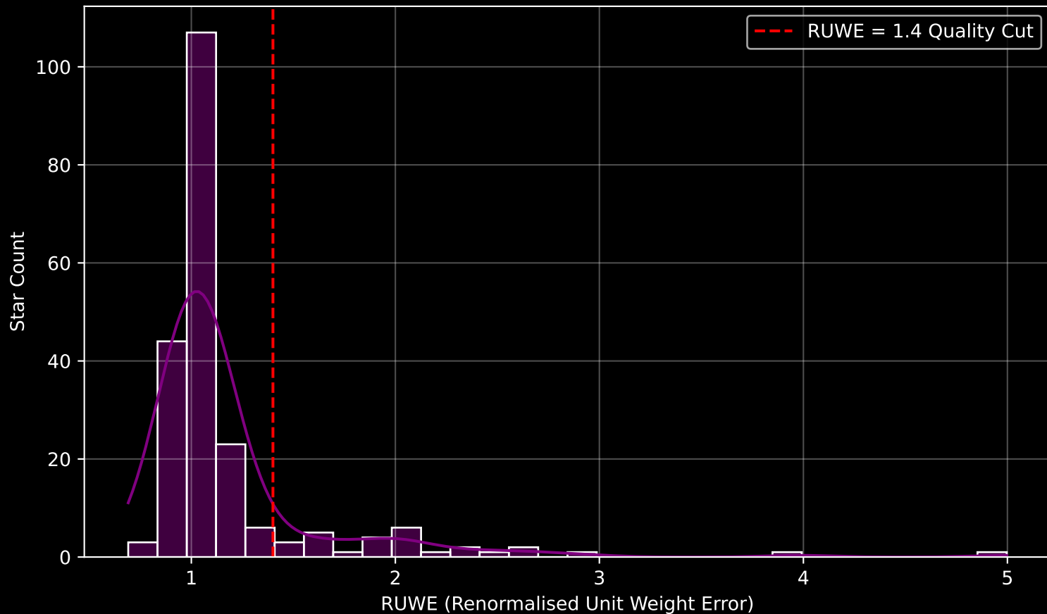
GAPOGEE DR17 Field [247+62_btx] RUWE Distribution (n= 211)
